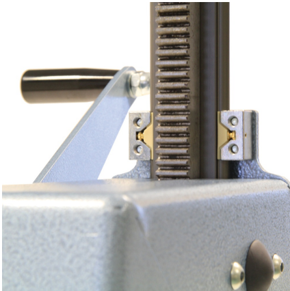
Detail of soil sampler rack and pinion mechanism
